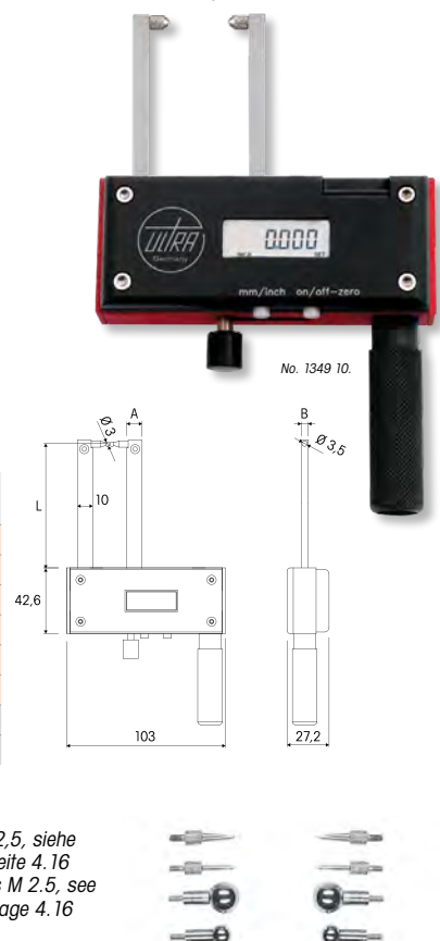
Messweg 25mm Measuring way 25mm
