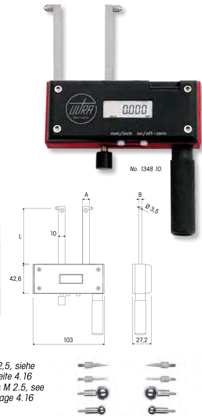
Messweg 25mm Measuring way 25mm
